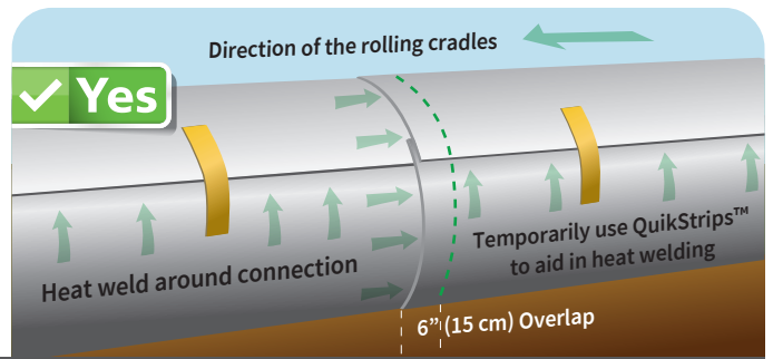
Method 2: Heat weld to seal
