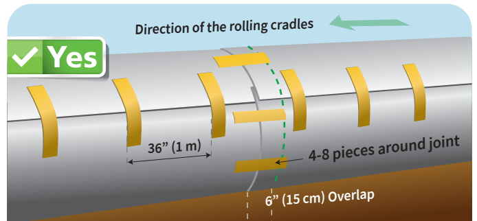
Method 1: QuikStrips™ are 36" (1 m) apart
