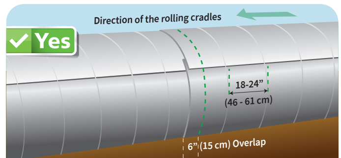
Method 3: Butyl or filament tape, 18-24" (46-61 cm)
