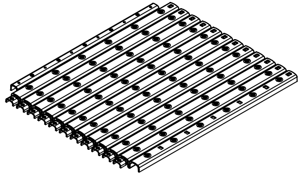
Isometric
