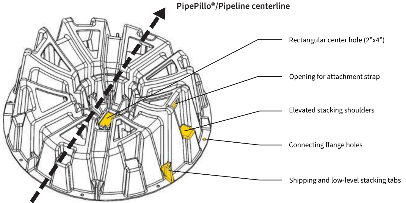
PipePillo® Pipeline Supports
